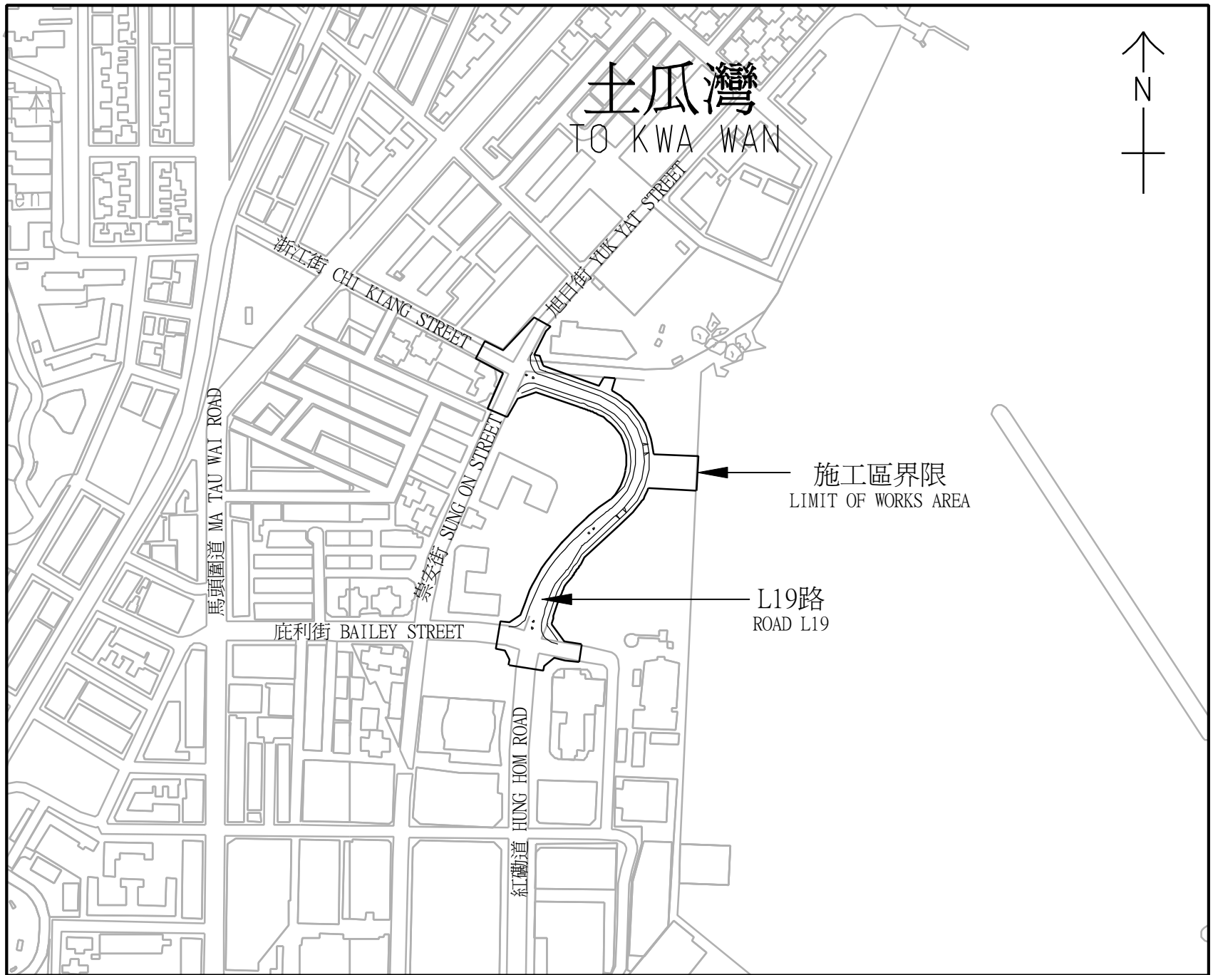
啓德機場北面停機坪的基礎設施 L19路建造工程及相關基建工程位置圖 Location Plan of Infrastructure at North Apron Area of Kai Tak Airport Road L19 and Associated Infrastructure Works
